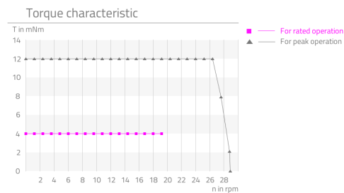
P-019 Curve measured with 5x nominal voltage and load inertia 6 \cdot 10E-9 \text{ kg/m}^2 in \frac{1}{4} micro steps.
