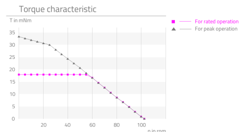
P-019 Curve measured with 5x nominal voltage and load inertia 6 \cdot 10E-9 kg/m 2 in \frac{1}{4} micro steps.
