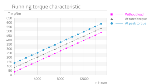
P-029 Curve measured with 5x nominal voltage and load inertia 6 \cdot 10E-9 kg/m 2 in ¼ micro steps.
